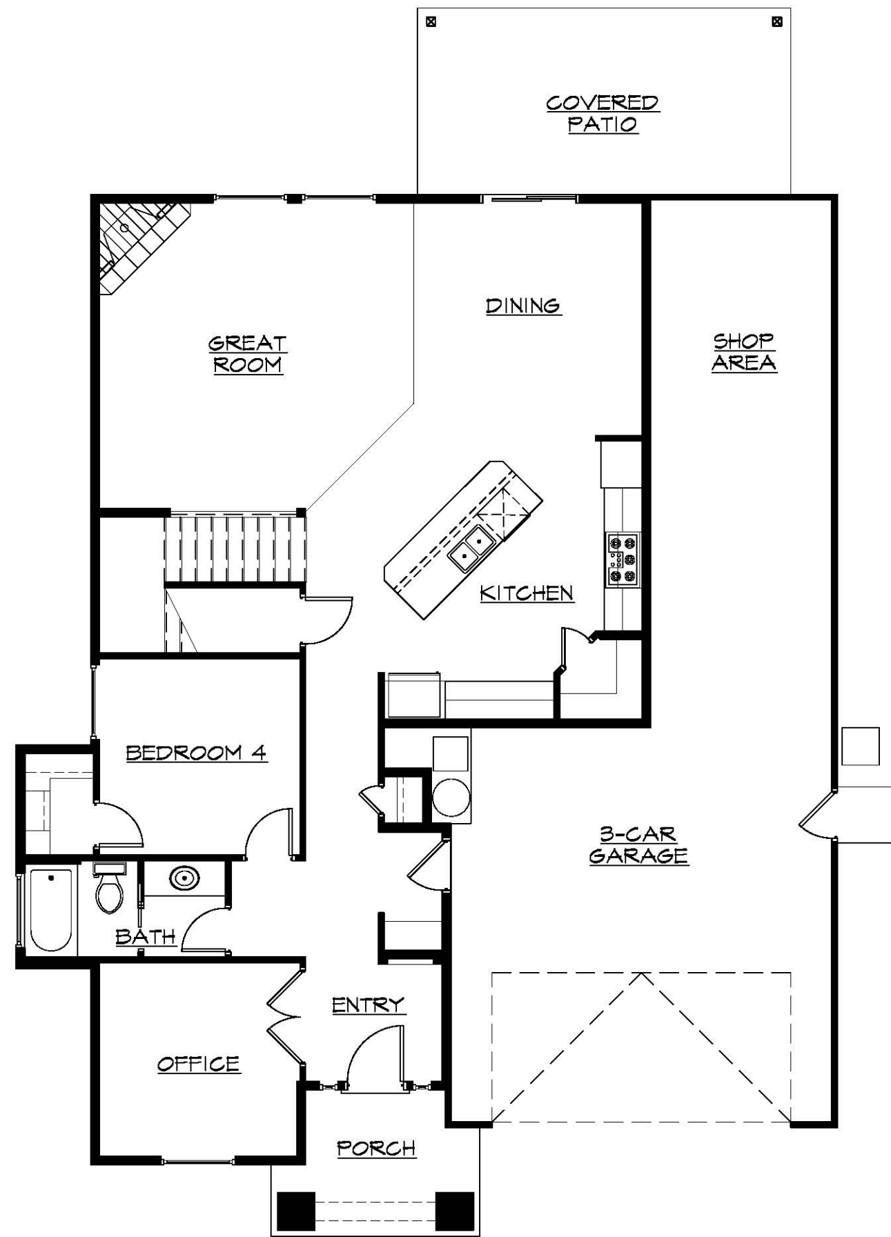
MAIN LEVEL FLOOR PLAN 1,315 S.F.
